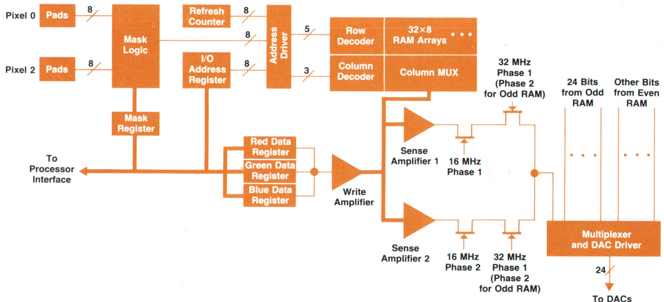
Fig. 4. Block diagram of even-pixel RAM on color map/video DAC chip.
