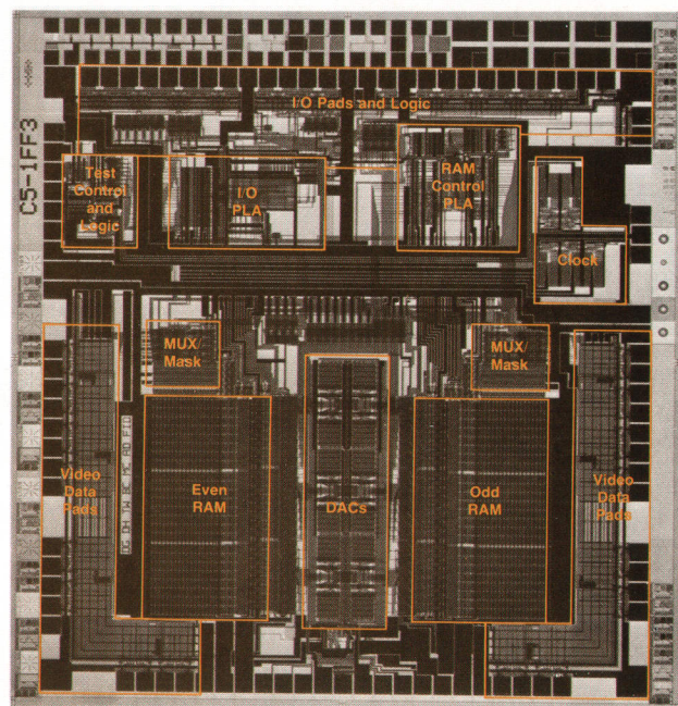
Fig. 3. Photograph of the color map/video DAC chip.
