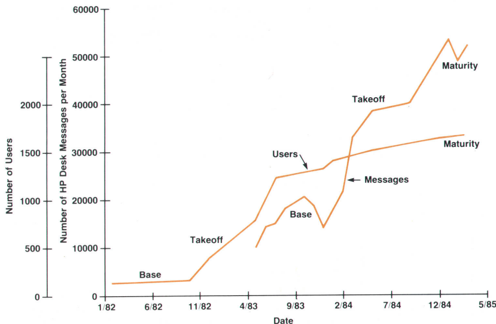
Fig. 13. Growth in number of users and number of messages processed in the HP Corporate Offices HP Desk network. Growth occurs in three phases, labeled base, takeoff, and maturity.
