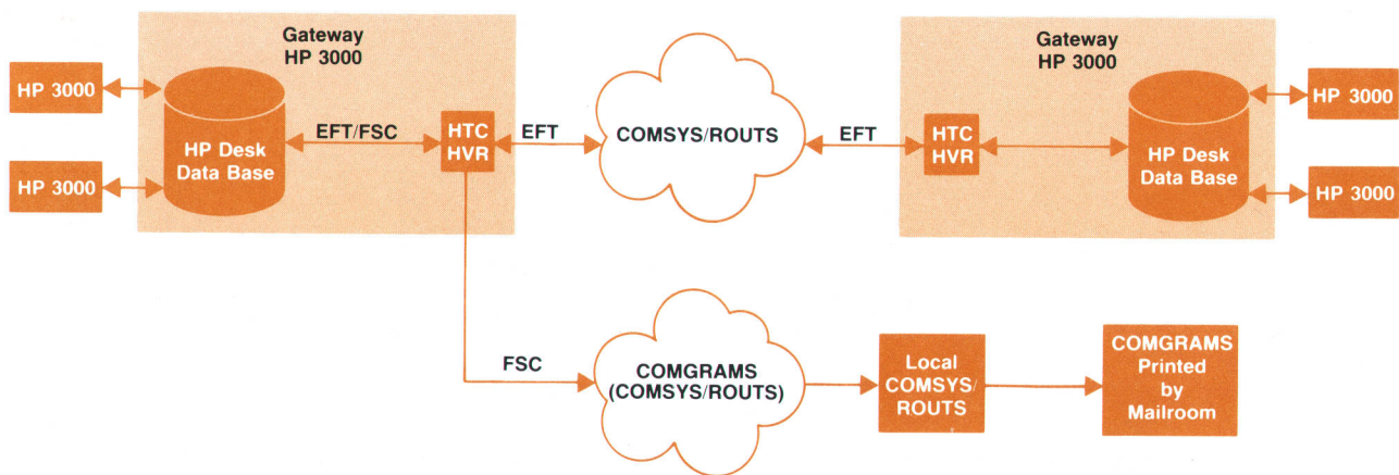
Fig. 7. HTC (HP Desk to COMGRAMS) and HVR (HP Desk via ROUTS) are examples of user-written utilities that use the EFT and FSC facilities of HP Desk.
