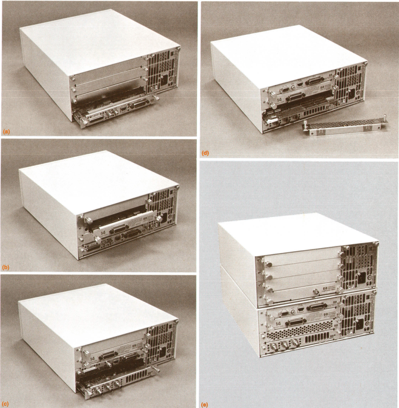
Fig. 2. (a) The minimum Series 300 configuration is the single-board computer. (b) Expand the system by adding the DIO card cage. This allows the addition of more memory, I/O cards, or accessory cards. (c) Upgrade with any of four optional graphics interfaces—high- or medium-resolution, color or monochrome. (d) Upgrade to the 68020 processor. This requires the DIO card cage for the HP-HIL board and memory. (e) Expand again with the DIO expander for a total of twelve DIO slots.
