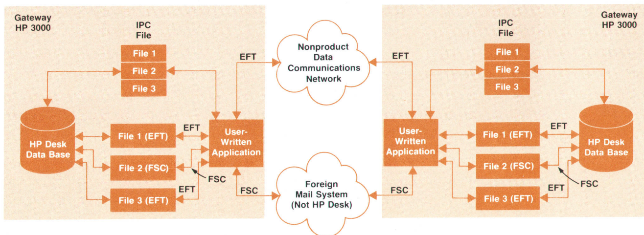
Fig. 6. How HP Desk uses EFT (external file transfer) and FSC (foreign service connection). An IPC (interprocess communication) file acts as a queue of all EFT and FSC files containing messages for various mailnodes.
